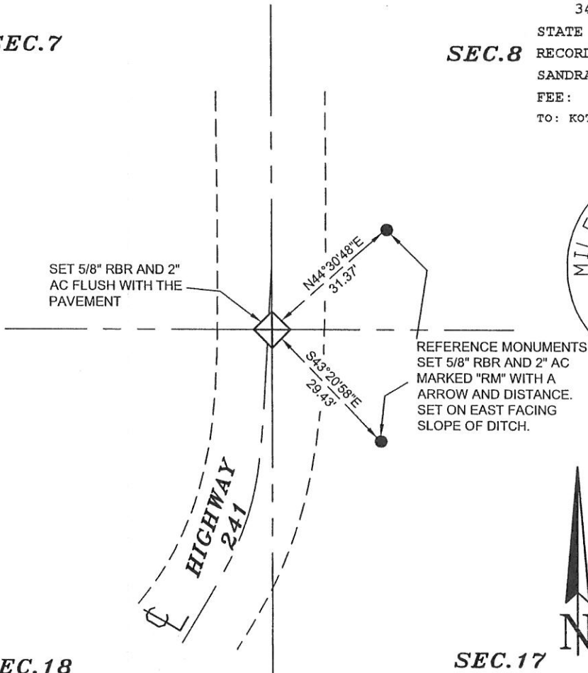
SKETCH OF CORNER
