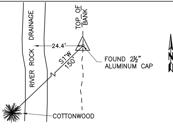
(Not to Scale) SKETCH OF CORNER
