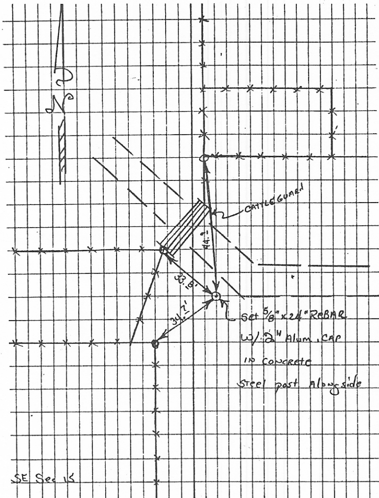
SKETCH OF CORNER
